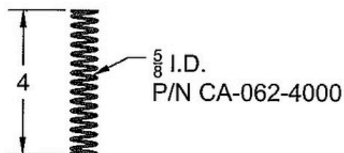
SPRING
