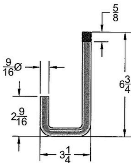
J-HOOK CA-56-3.25
